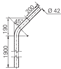
LMZ 48 - 1900/190 - FT
