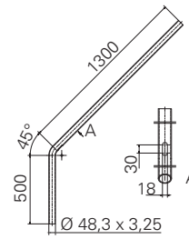
LMW 48 - 500/1300 - FT
