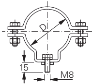
Pipe clamp
