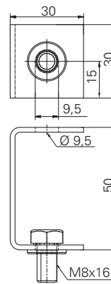
C-bracket
