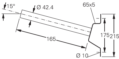
Wandarm W27
