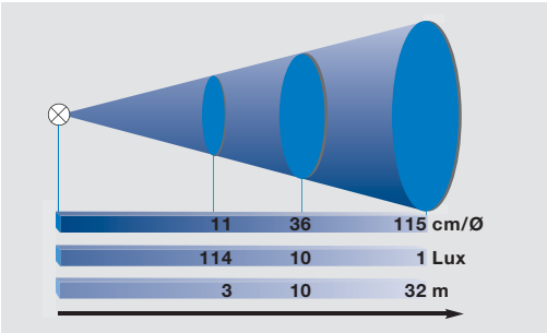
Range-diagram HE 9 Basic
