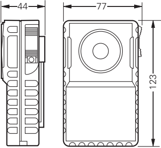
Dimension drawing HE 5 EN
