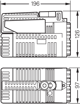
Dimension drawing HE 9 Basic
