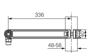
Bracket pole mounting
